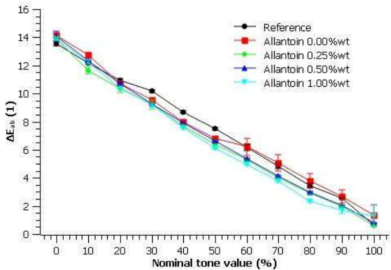
Figure 5: Black colour difference after accelerated thermal ageing depending on nominal tone value
