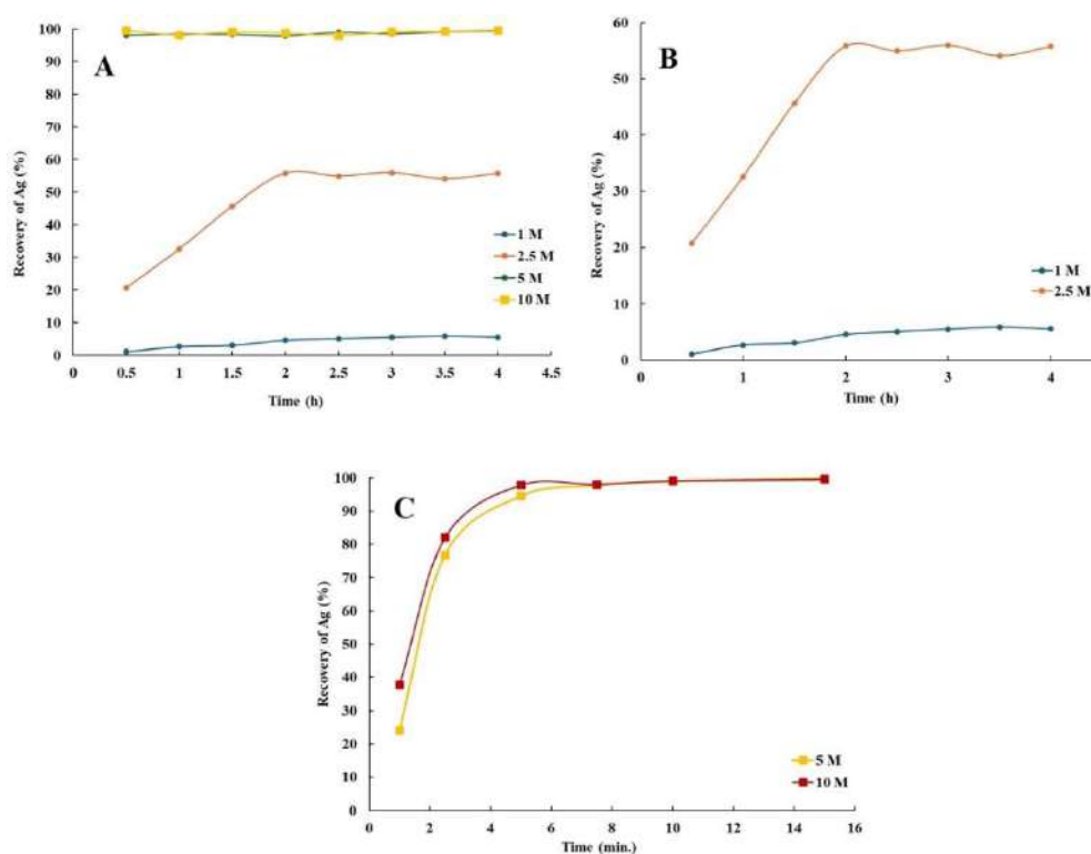
Figure 7: Effect of treatment time with (A) all HNO 3 concentrations (B) with 1.0 M and 2.5 M HNO 3 and (C) with 5.0 and 10.0 M HNO 3 on recovery of silver
