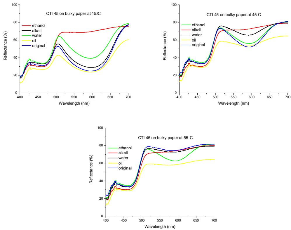
Figure 4: Spectral reflectance curves of CTI 45 measured at three different temperatures on bulky paper
