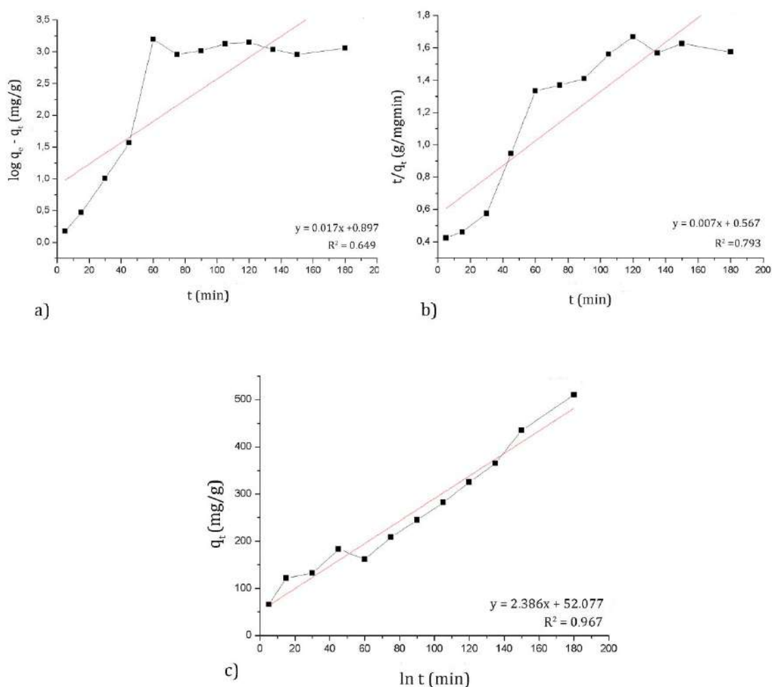
Figure 3: The plots of modelling experimental data: a) pseudo-first order, b) pseudo-second order, c) Elovich model
