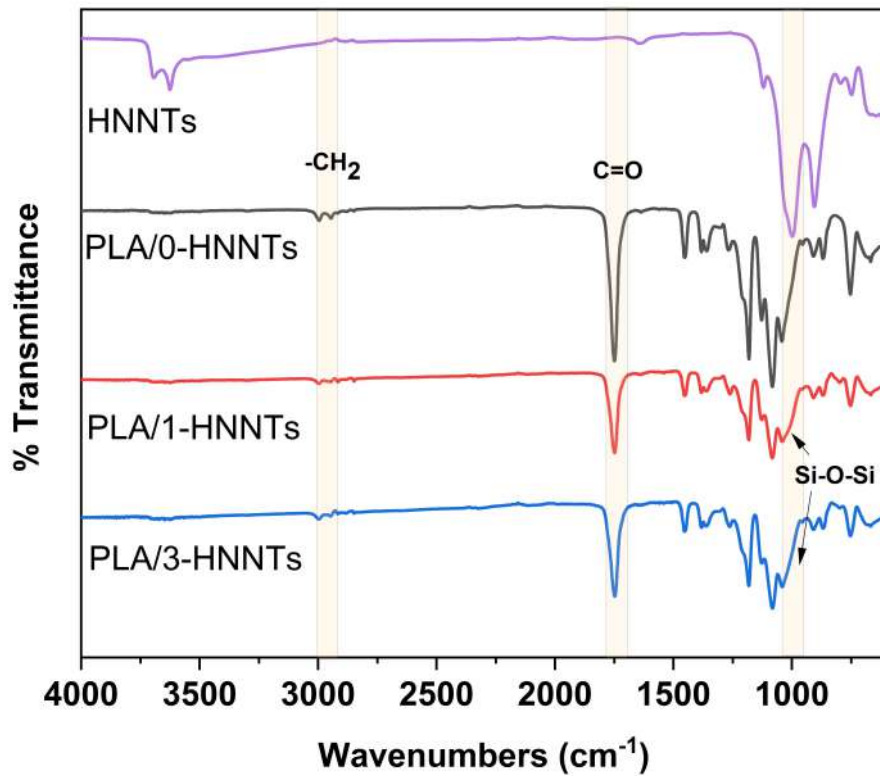
Figure 2: FTIR spectra of PLA/HNNTs nanocomposite loaded with 0, 1, and 3, wt% HNNTs. The spectrum for HNNTs is shown for comparison
