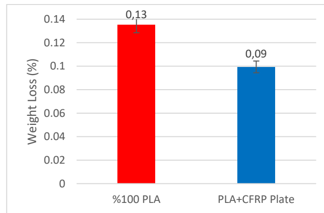
Figure 10: Abrasion test results
