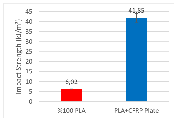
Figure 8: Izod impact test results
