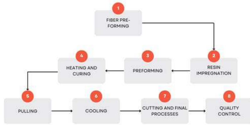
Figure 1: CFRP plate production method flow chart
