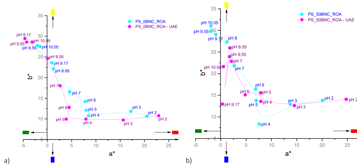
Figure 7: CIE a^*/b^* values for potato starch-based films produced without and with UAE, a) PS_0BNC, b) PS_50BNC
