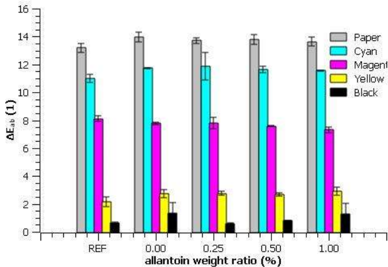
Figure 4: Colour difference of paper and full tone on coated samples after accelerated thermal ageing
