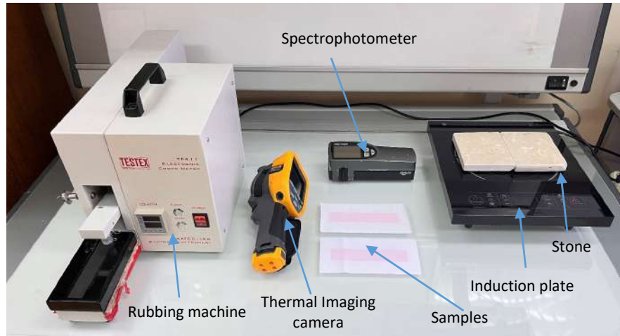
Figure 1: Experimental setup
