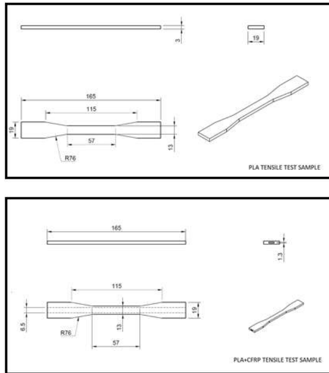
Figure 3: Technical drawing of the tensile specimens
