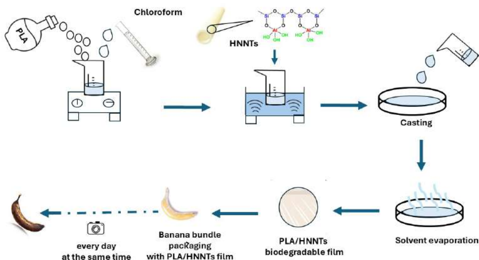
Figure 1: The preparation scheme of PLA/HNNTs nanocomposite packaging film
