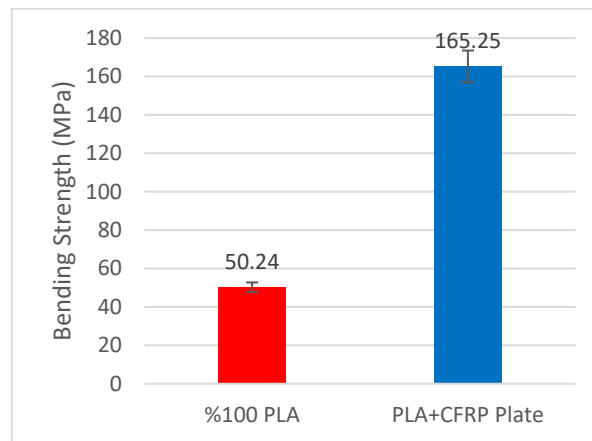
Figure 13: Three-point bending test results
