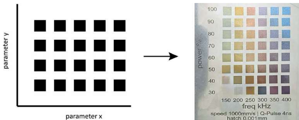
Figure 1: Laser parameter matrix for color testing
