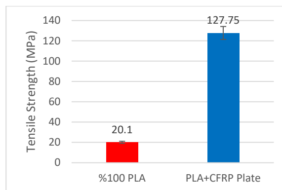
Figure 11: Tensile test results
