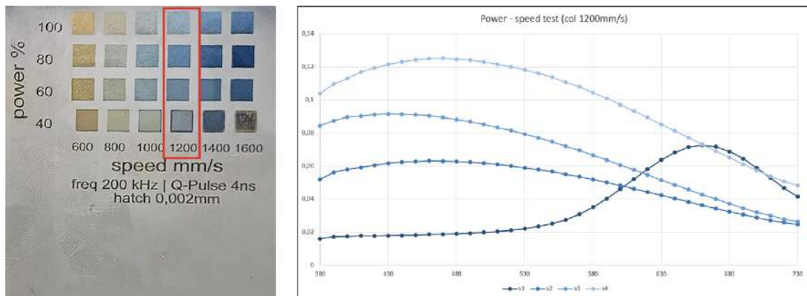
Figure 5: Power-speed test results
