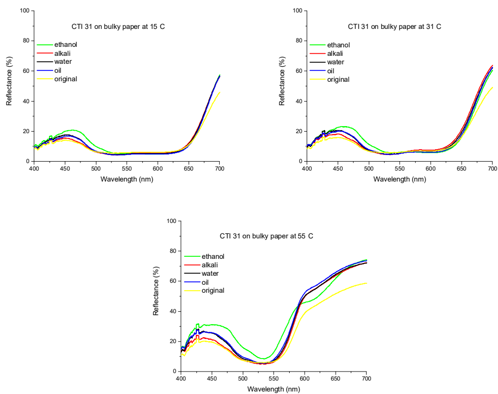
Figure 2: Spectral reflectance curves of CTI31 measured at three different temperatures on bulky paper
