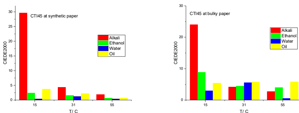
Figure 6: CIEDE2000 colour difference observed on CTI45 samples when exposed to different chemicals
