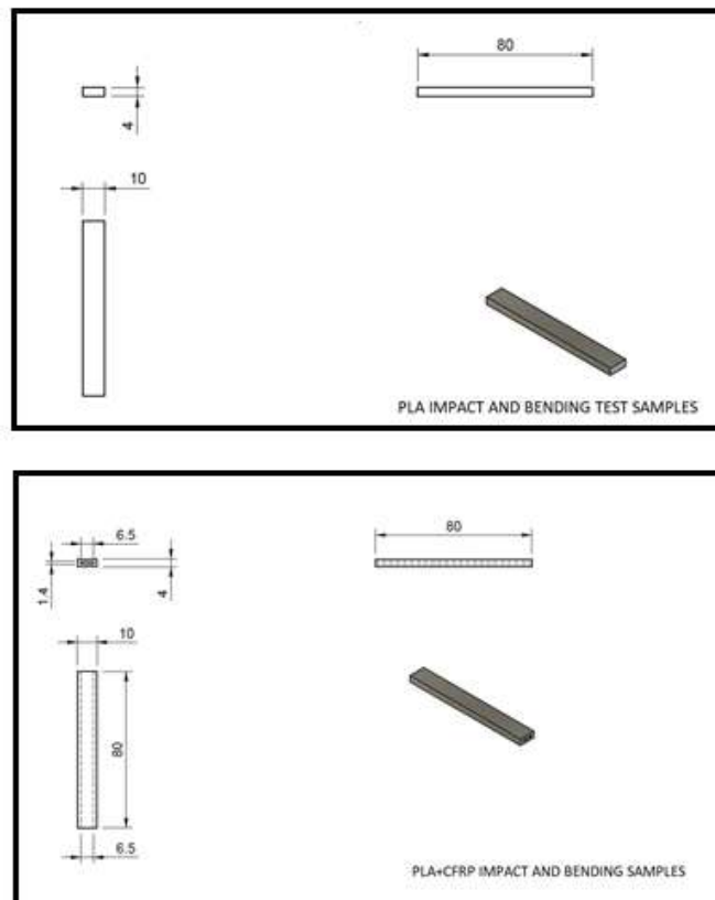
Figure 4: Technical drawing of the impact and bending test specimens
