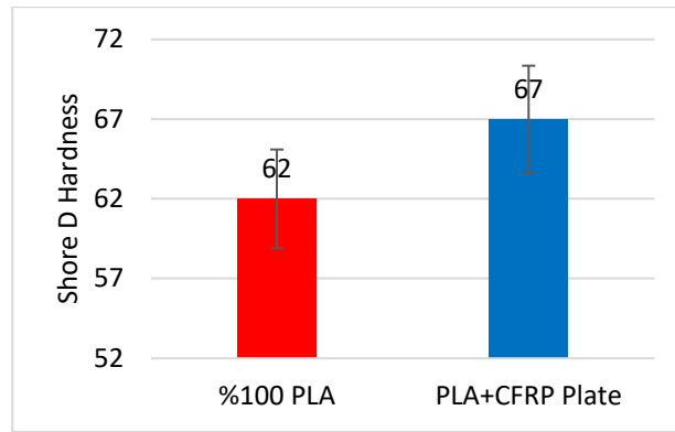
Figure 9: Shore D hardness test results
