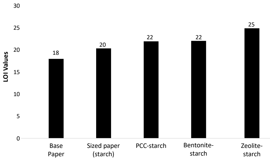
Figure 5: LOI values of base paper PCC-starch, bentonite-starch, and zeolite-starch coatings
