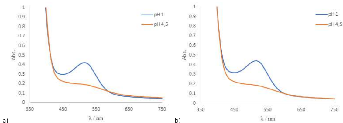
Figure 2: UV-Vis absorption spectra of anthocyanin extracts, a) untreated ROA and b) ultrasound treated ROA (ROA-UAE)
