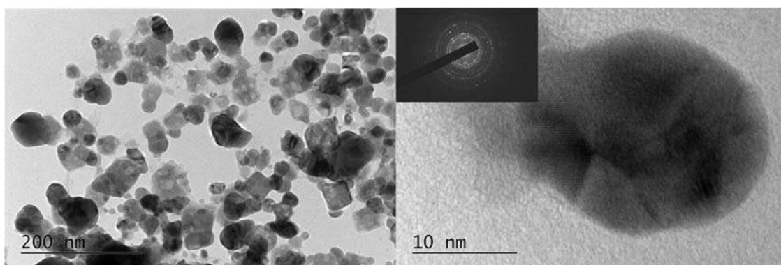
Figure 2: TEM images and the corresponding electron diffraction patterns of silver nanoparticles obtained with Sideritis scardica extract
