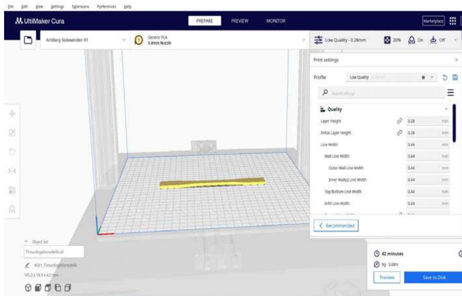
Figure 5: Transfer and adjustment in the Slicing program
