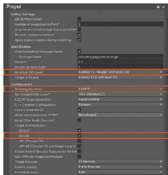
Figure 1: Player Settings
