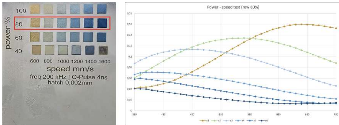
Figure 4: The influence of laser speed on surface coloration
