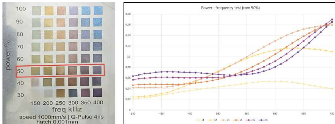
Figure 2: Power-frequency test results
