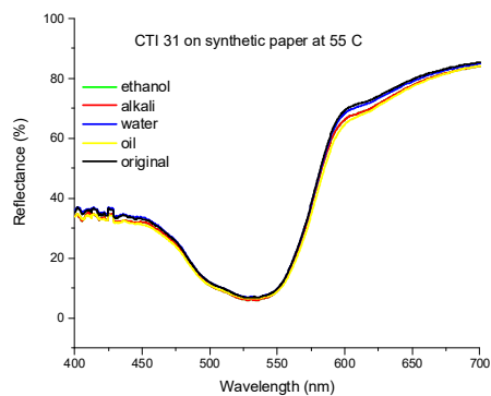
Figure 1 (part 2): Spectral reflectance curves of CTI31 measured at three different temperatures on synthetic paper
