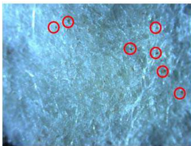
Figure 5: Stainless steel particles, circled in red, on the filtrated paper fiber residues
