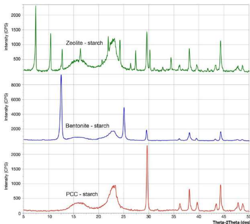
Figure 6: X-Ray diffractograms (XRD) of zeolite doped starch hybrid film (green), bentonite doped starch hybrid film (blue), \text{CaCO}_3 (PCC) doped starch hybrid film (red)
