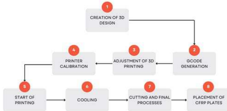
Figure 2: Production flow chart of PLA composite samples containing CFRP plate
