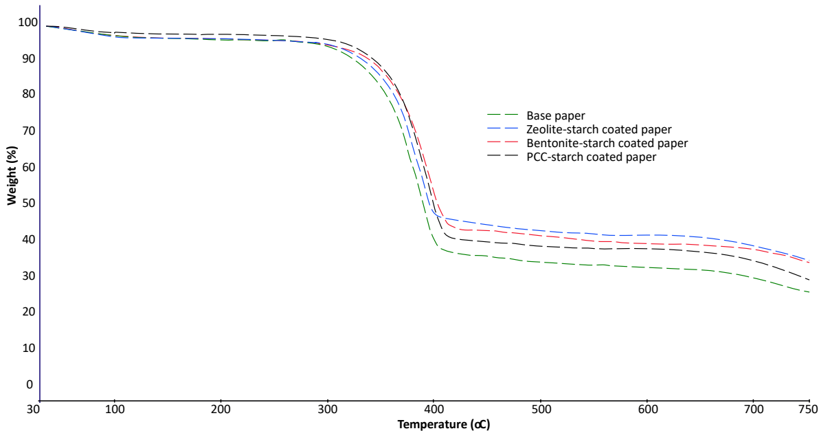
Figure 4: TGA thermograms of base paper PCC-starch, bentonite-starch, and zeolite-starch coatings
