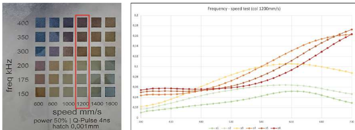
Figure 7: Frequency-speed test results at 1200mm/s
