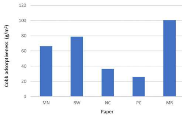
Figure 2: The results of Cobb absorptiveness ( t = 60 s) of the papers
